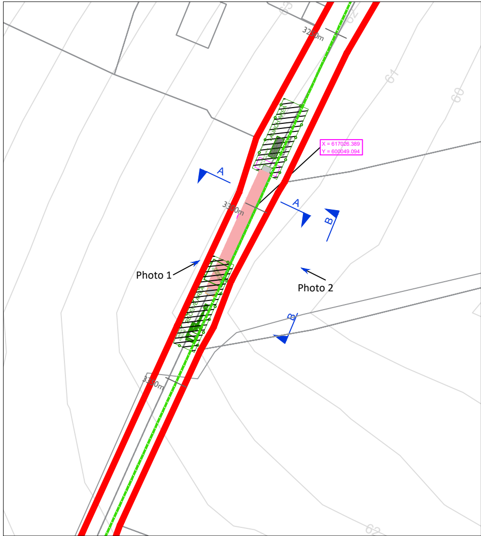
Plan View Watercourse 1 Scale ; 1:1000
